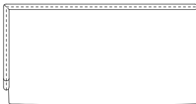
sofá C138 1BR ESQUERDO 175x90x65cm (LxPxA) almofadas: 2x und. decorativa 50x50cm 2x und. decorativa 55x55cm
